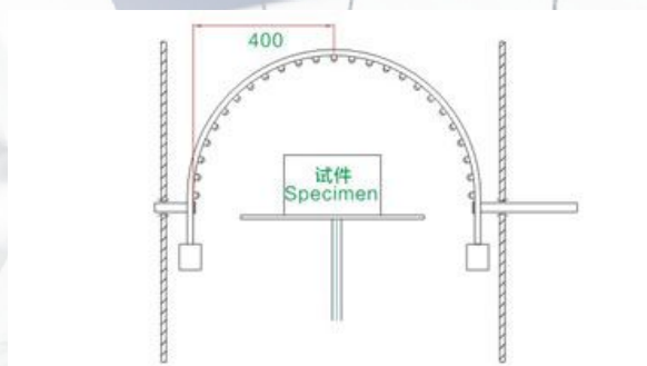
IPX3摆管Swing pipe IPX4摆管Swing pipe
